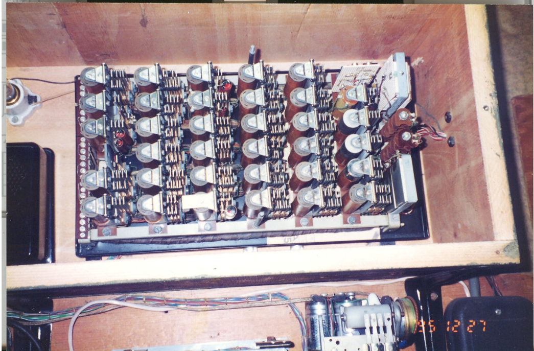
Frank D Reese's ATEA PABX built into a wooden box
