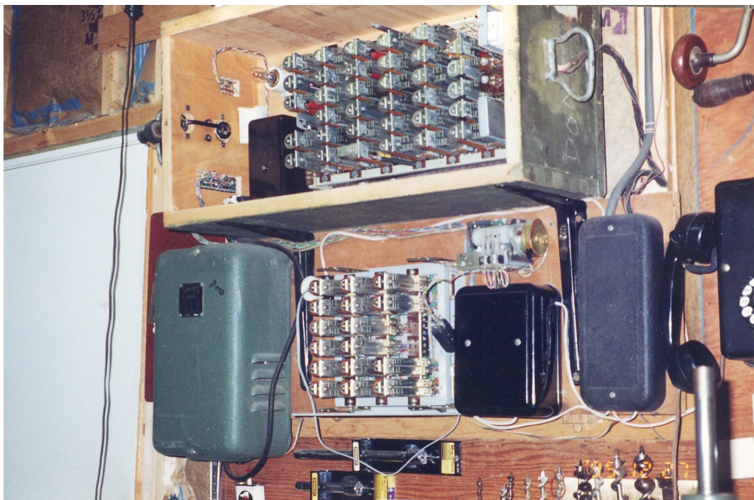
Frank D Reese's ATEA PABX with expansion to 8 lines and DTMF receiver
