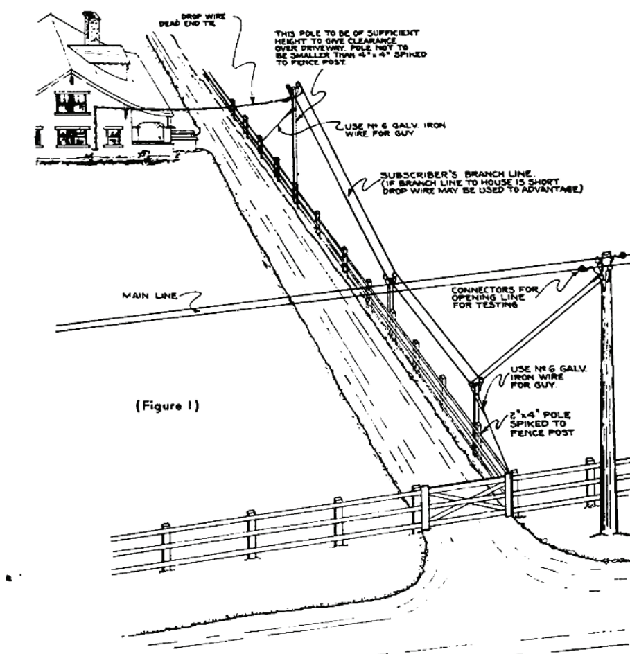
Fig. 6: Pacific Bell instructions to setup a rural network
